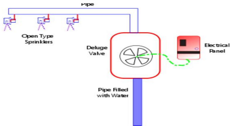
Figure 24:Deluge valve
